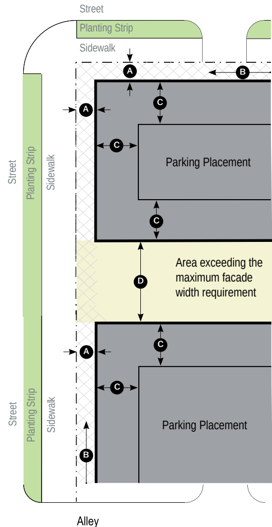
Building Plan
