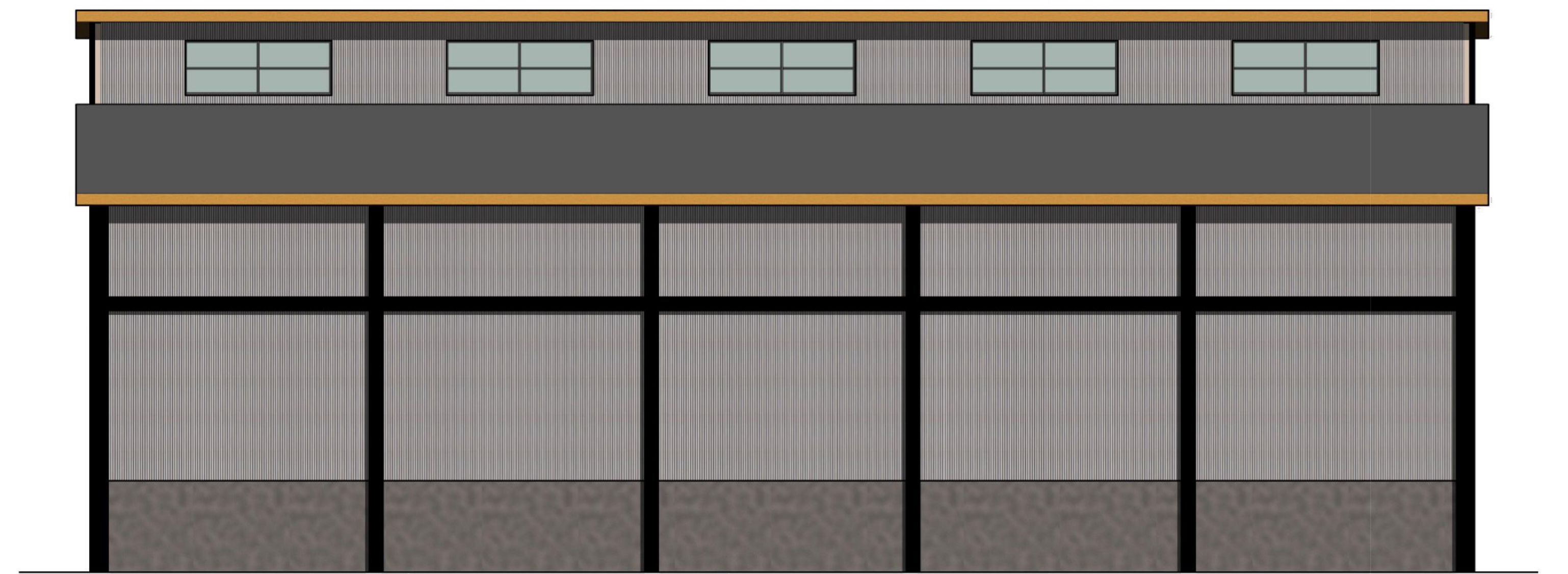
④ SIDE ELEVATION B 3/32" = 1'-0"
