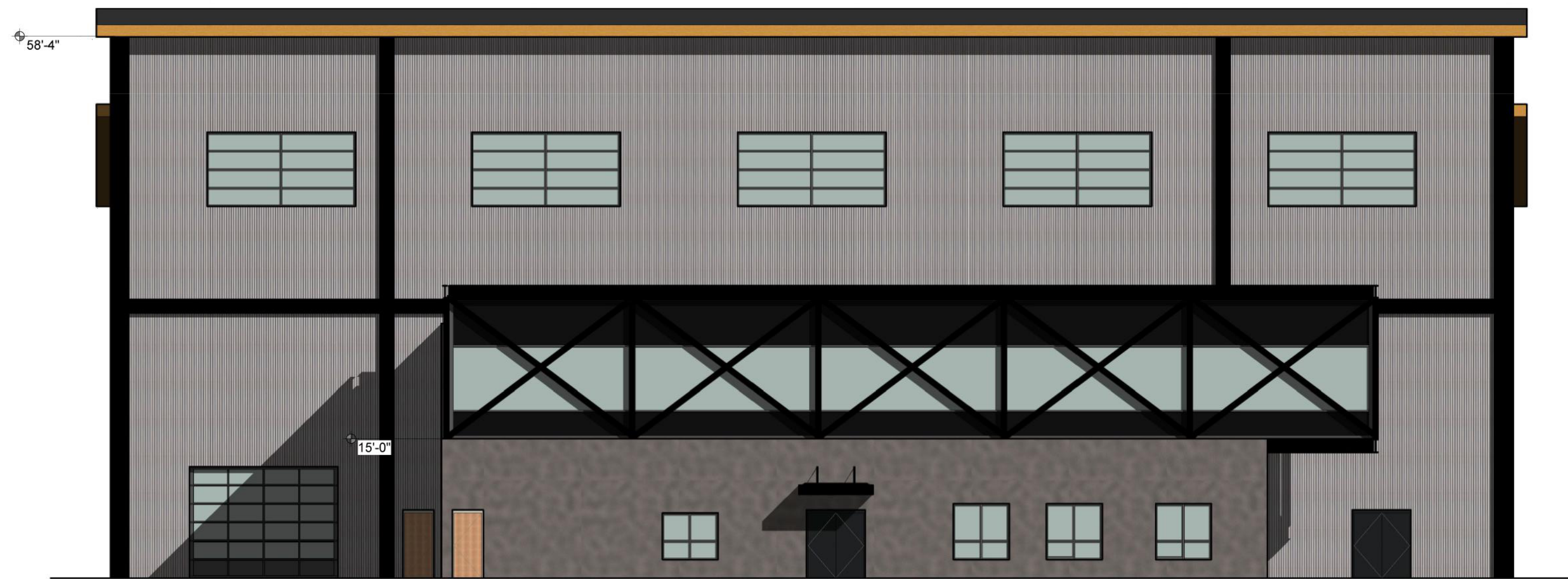
① SIDE ELEVATION A 3/32" = 1'-0"
