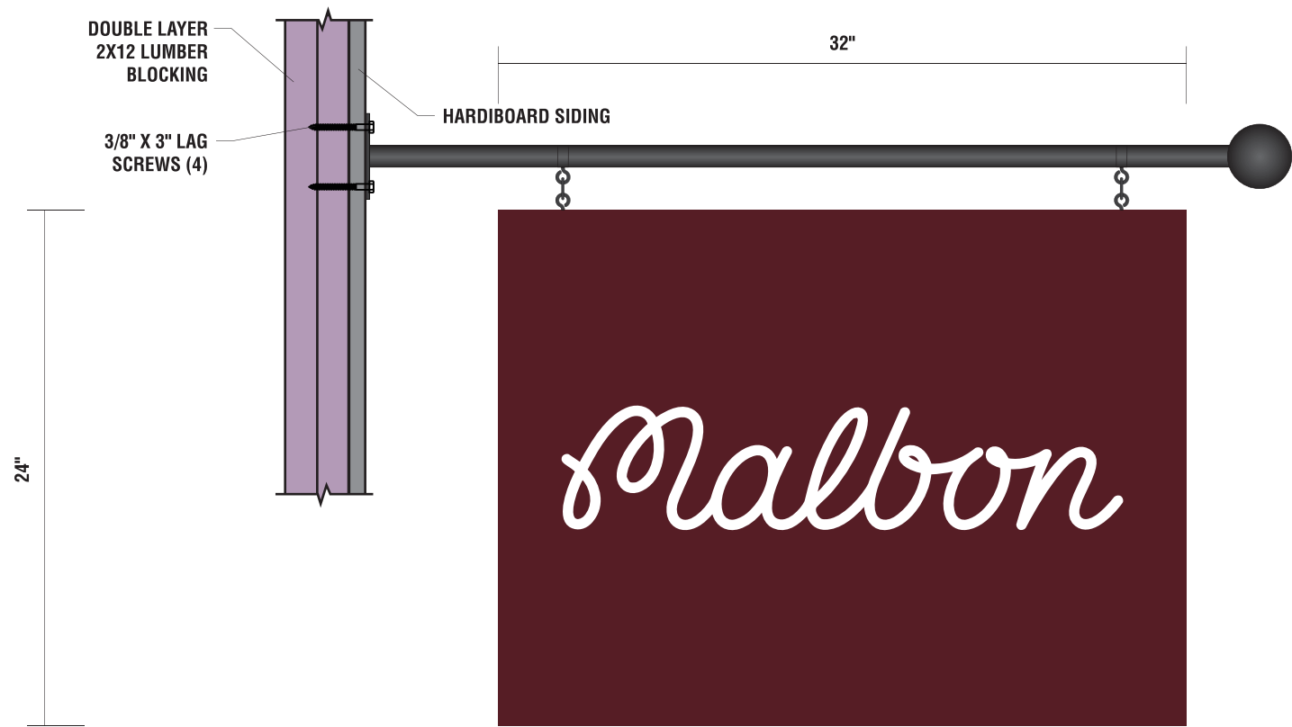
3 FRONT VIEW - BLADE SIGN SCALE: 1-1/2" = 1'-0"
