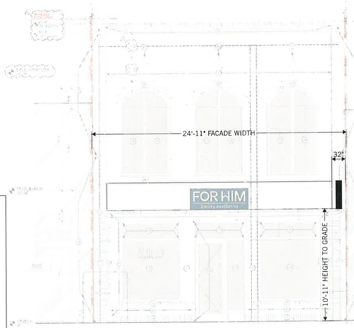
1 EXTERIOR ELEVATION - CHARLOTTE PIKE - RENOVATED SCALE: 3/16"=1'0"
