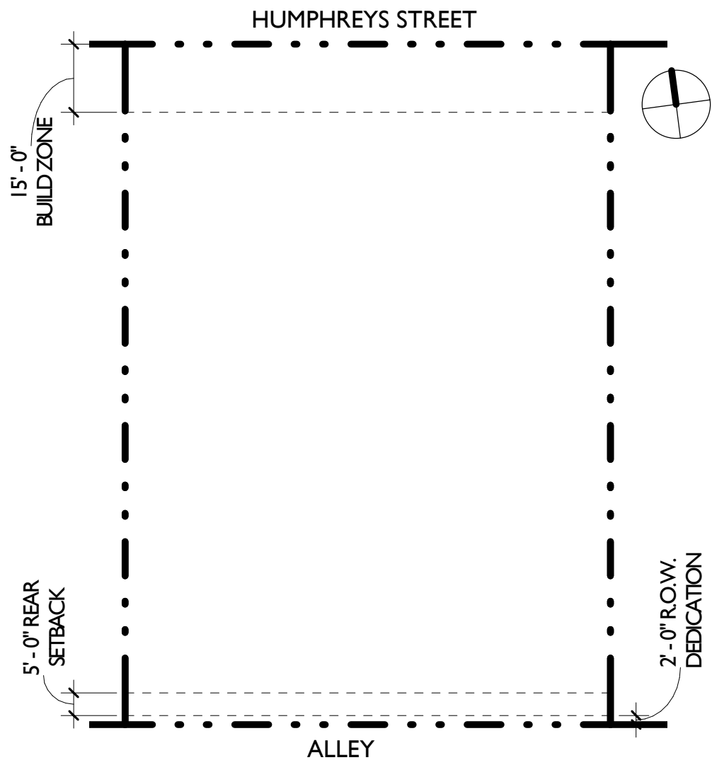
SITE DIAGRAM
