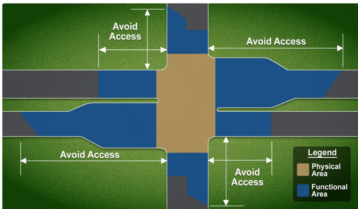
Figure 3-3: Intersection Functional Area
