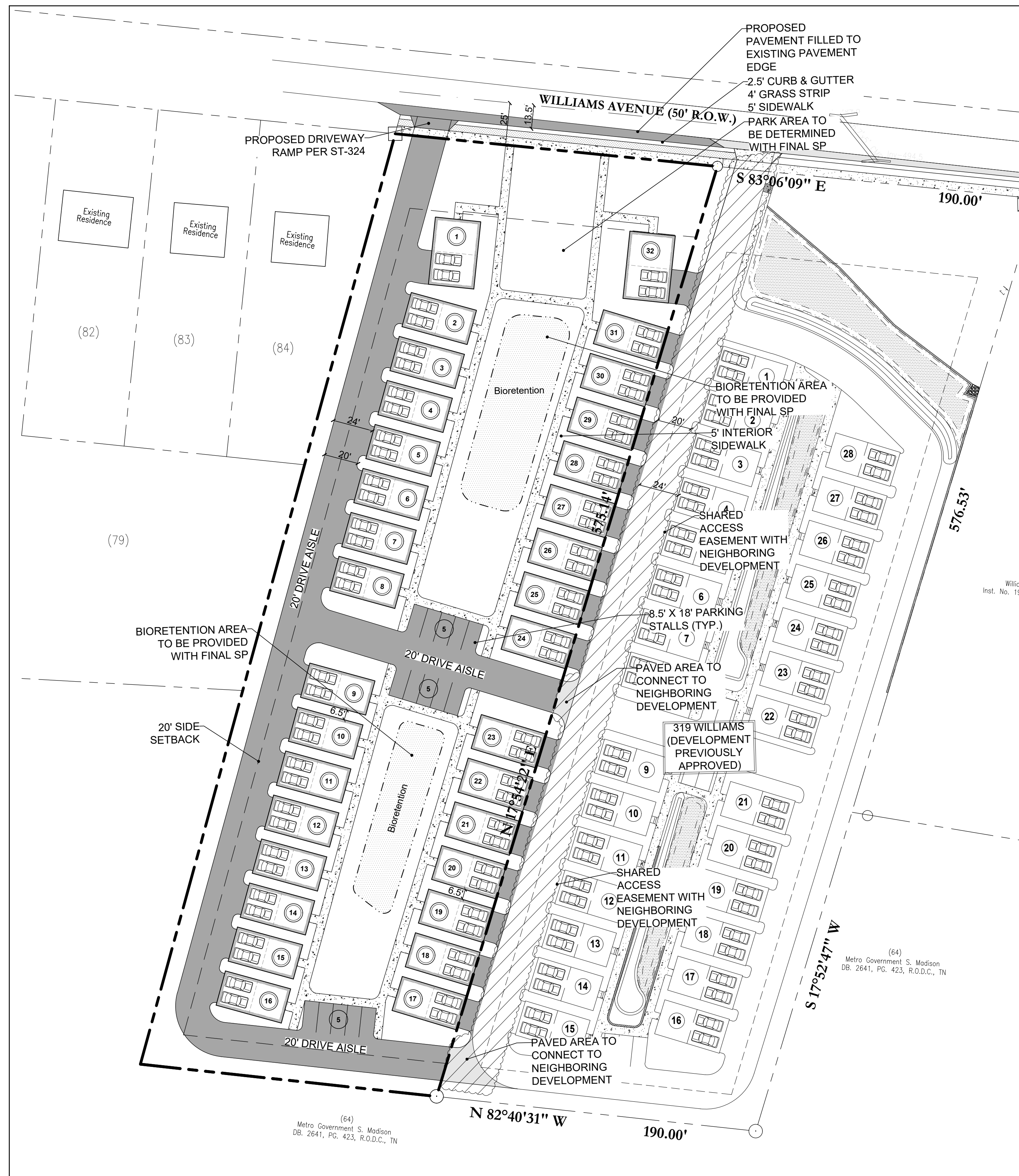
SP Plan (1"=40')
